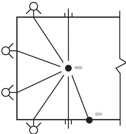
Fig. 3 - Deep-End Pattern with SwingJets
