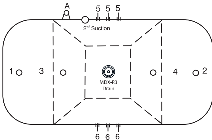
Vanquish pools with downjet option
