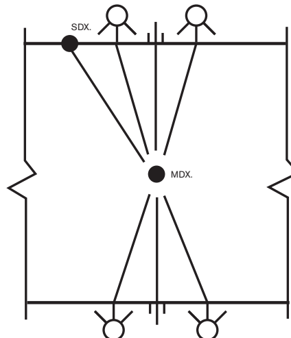
Fig. 4 - Center-Depth Pattern with SwingJets
