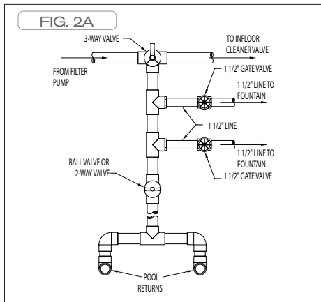
With Infloor Cleaning System Figure 2A
