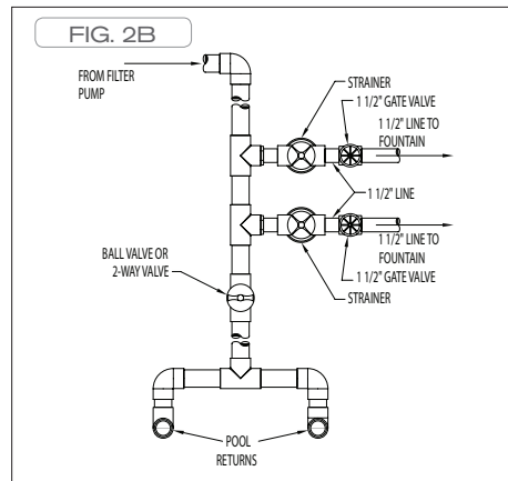
With Wall Returns – No Infloor System Figure 2B
