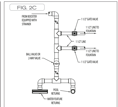
With Wall Returns & Water Features Figure 2C
